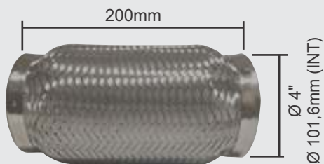
FLEXIVEL MALHA Ø INT. 4" (101,6mm) X 200mm S/ TUBO INT. GRAMPEADO
