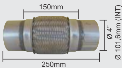
FLEXIVEL MALHA DUPLA Ø INT. 4" (101,6mm) X 150mm X 250mm
