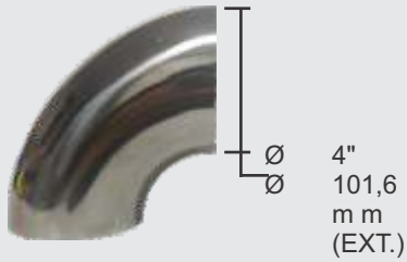
CURVA INOX 90° Ø4" (101,6mm) X 1,20mm
