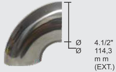
CURVA INOX 90° Ø4.1/2" (114,3mm) X 1,20mm
