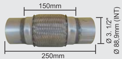
FLEXIVEL MALHA DUPLA Ø INT. 3. 1/2" (88,9mm) X 150mm X 250mm
