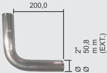
CURVA INOX - 90° Ø2" (50,8mm) X 1,20mm X 200mm
