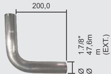
CURVA INOX - 90° Ø1.7/8" (47,6mm) X 1,20mm X 200mm
