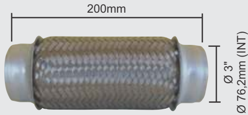
FLEXIVEL MALHA Ø INT. 3" (76,2mm) X 200mm S/ TUBO INT. GRAMPEADO
