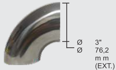
CURVA INOX 90° Ø3" (76,2mm) X 2,0mm
