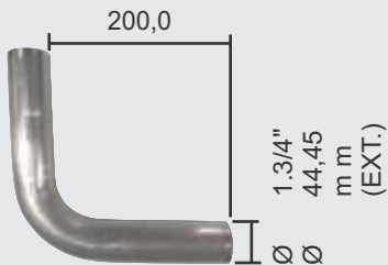
CURVA INOX - 90° Ø1.3/4" (44,45mm) X 1,20mm X 200mm
