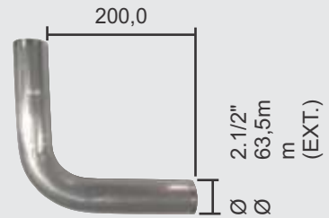
CURVA INOX - 90° Ø2.1/2" (63,5mm) X 1,20mm X 200mm
