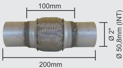
FLEXIVEL MALHA DUPLA Ø INT. 2" (50,8mm) X 100mm X 200mm
